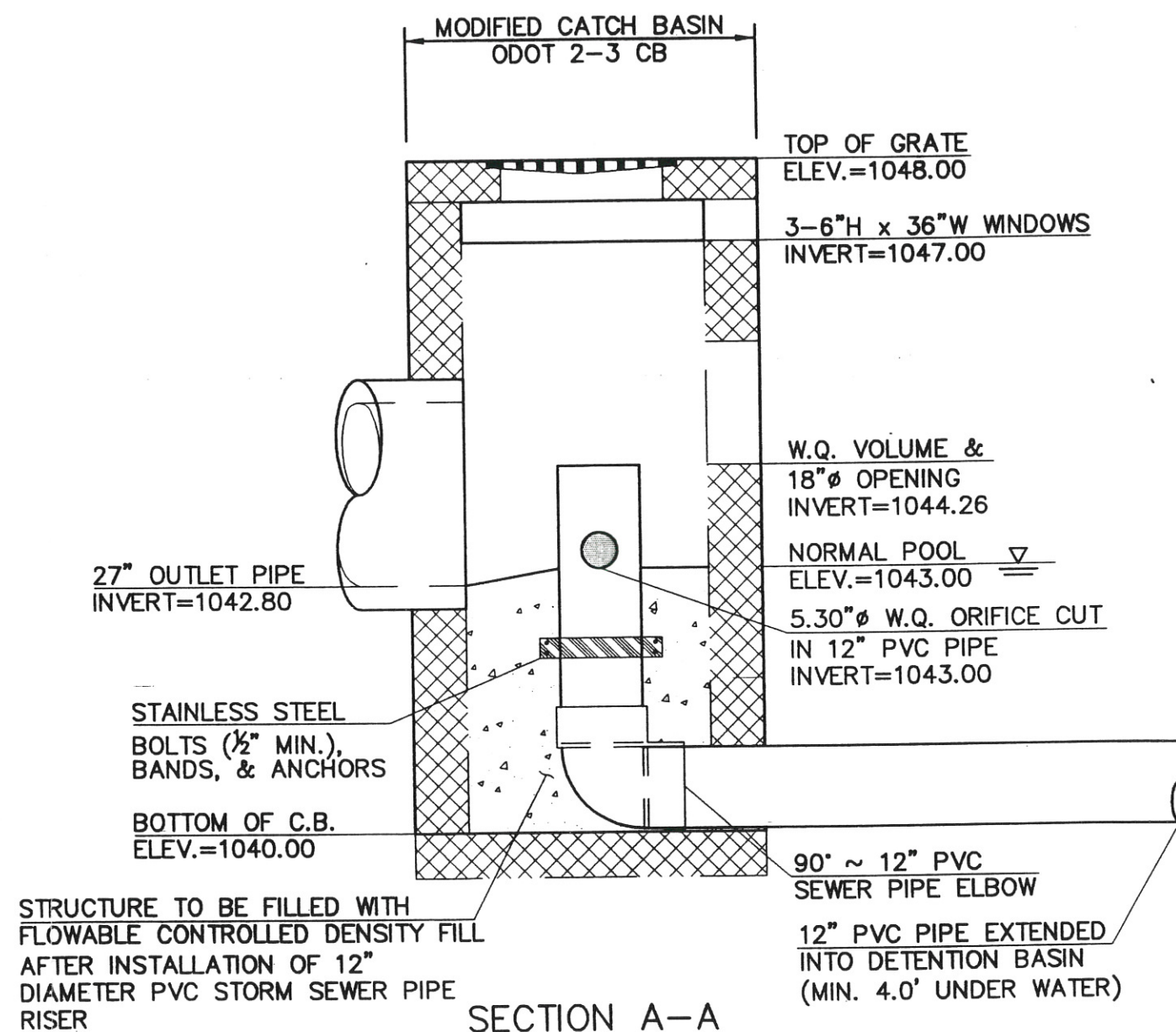
#11 BASIN OUTLET STRUCTURE DETAIL NOT TO SCALE
