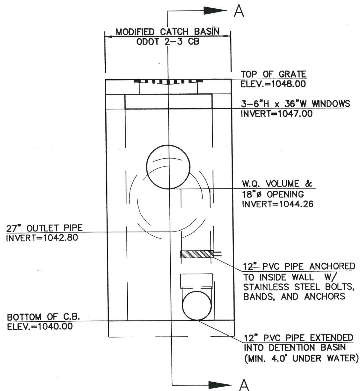
#11 BASIN OUTLET STRUCTURE DETAIL NOT TO SCALE
